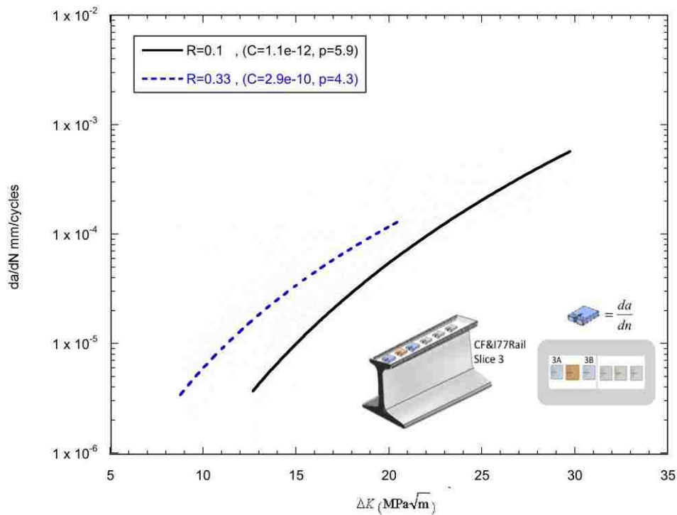
Figure 82 – Comparison of horizontal fatigue crack growth rates at two different R-ratios in Slice #3 of CF&I77 rail. R=0.1 and R=0.33 .
