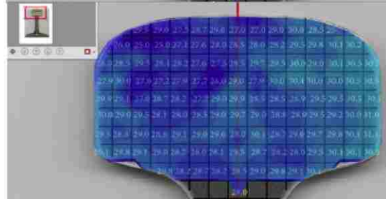
Figure 10 – Contour plots showing hardness variation in the rail heads using the same HRC scale.
